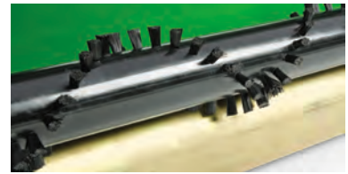
Rear roller power brush Prevents accumulation of grass clippings and other debris on the rear roller.
