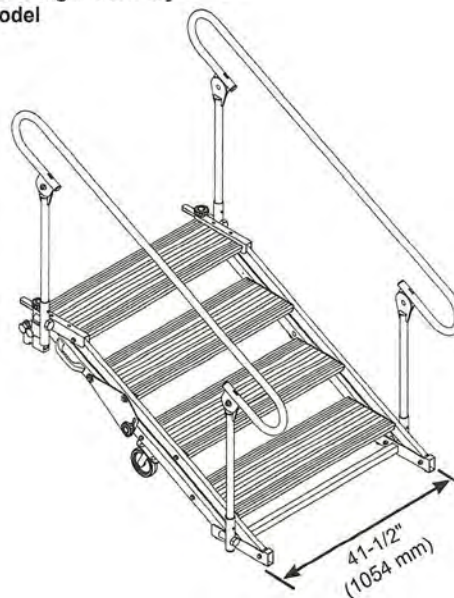
Adjustable Height Stairway 4-Step Model
