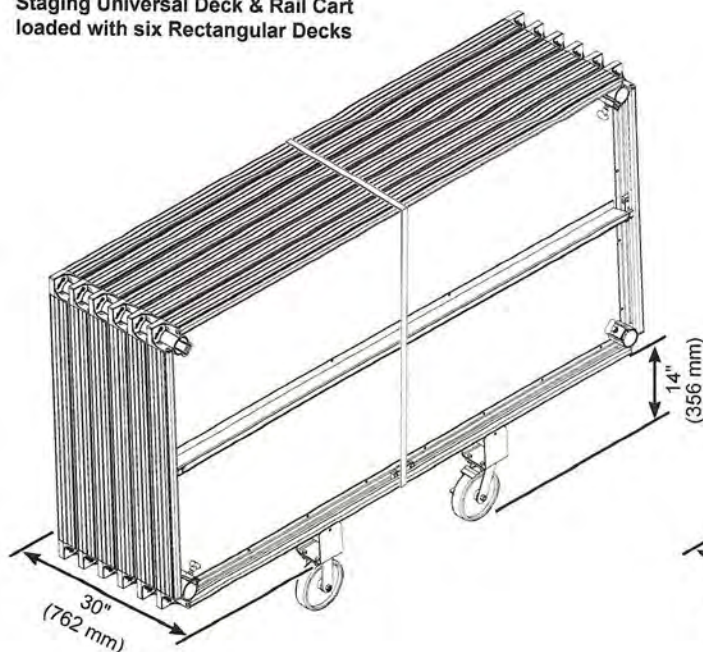
Staging Universal Deck & Rail Cart loaded with six Guardrails
