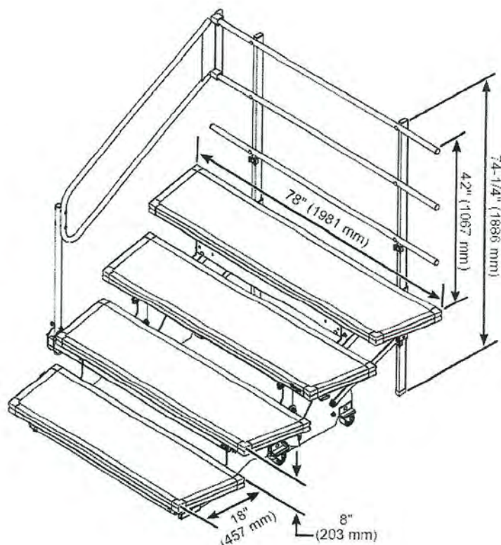
4-Step Riser with Optional Side Rail
